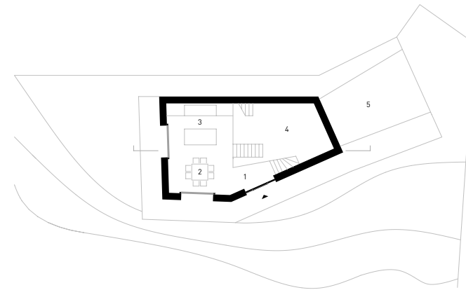
Erdgeschoss_piano terra
