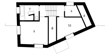
Obergeschoss_primo piano
